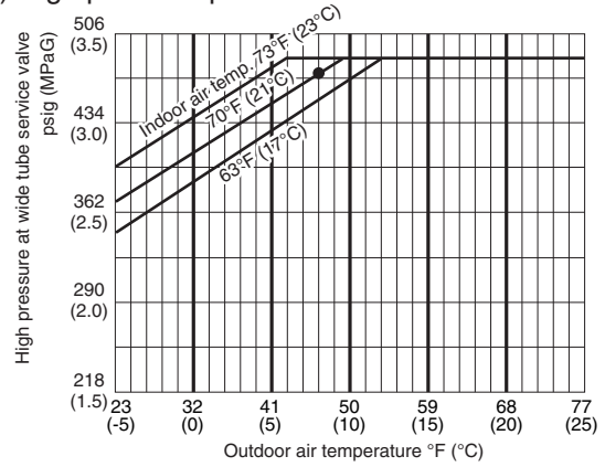
(2) Operating current performance chart
